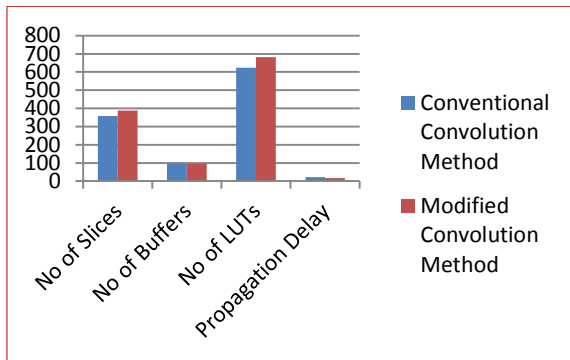
Figure 5 Graph between the Conventional and Modified Linear Convolution Technique
