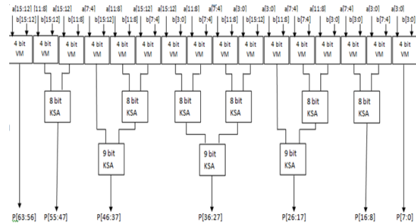
Figure 3 A 4 bit high speed linear convolution
