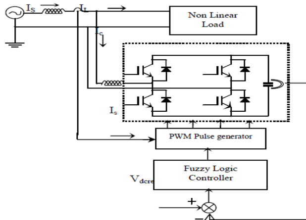
Figure 3 Block diagram of PI/Fuzzy controlled improved power quality converter
