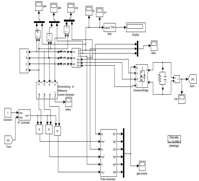
Figure 5 Simulated power circuit for PI controlled improved power quality converter
