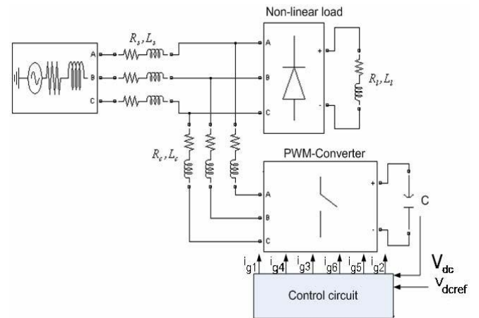
Figure 2 (a) Active filter system
