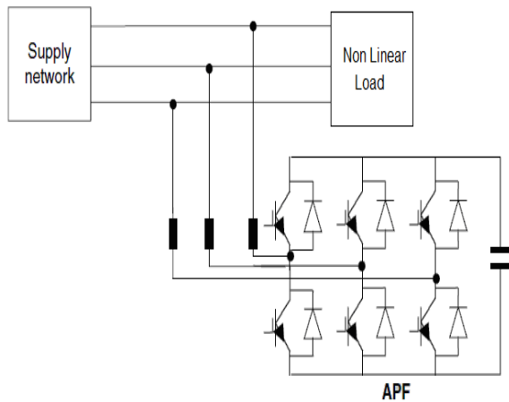
Figure 1 Active power filter connected with transmission line
