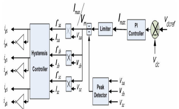
Figure 2 (b) Active filter system using PI controller
