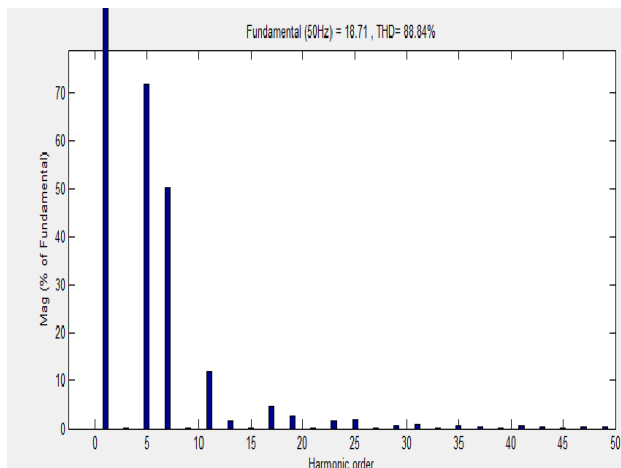
Figure 7 Harmonics spectrum without controller
