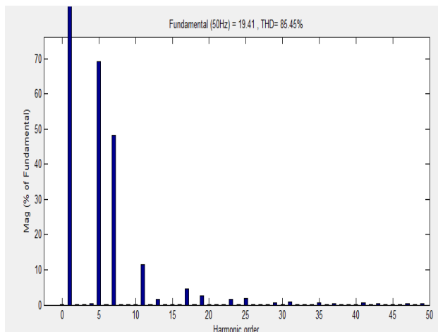
Figure 8 Harmonics spectrum with PI controller
